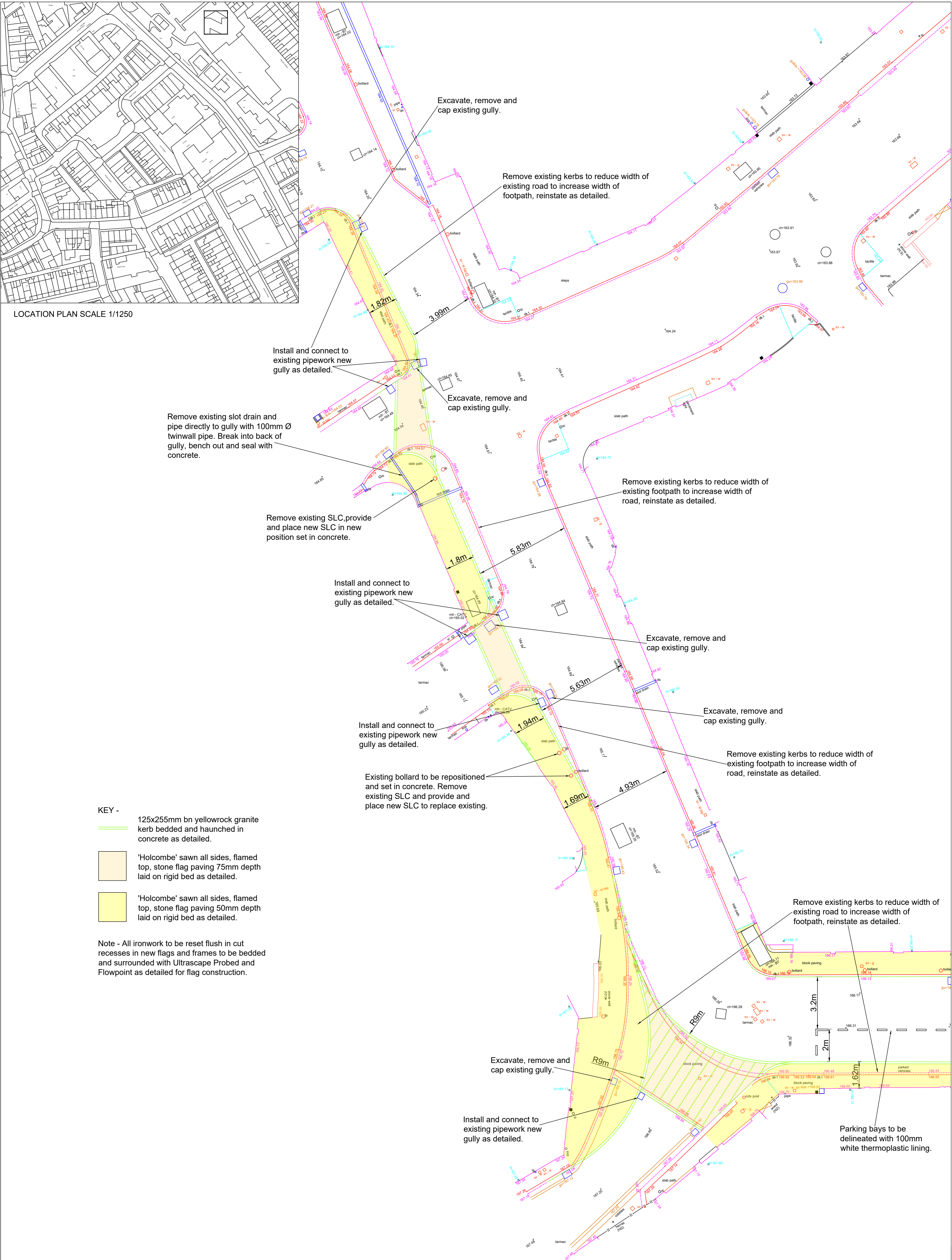
SCHEME DRAWING SCALE 1/100
