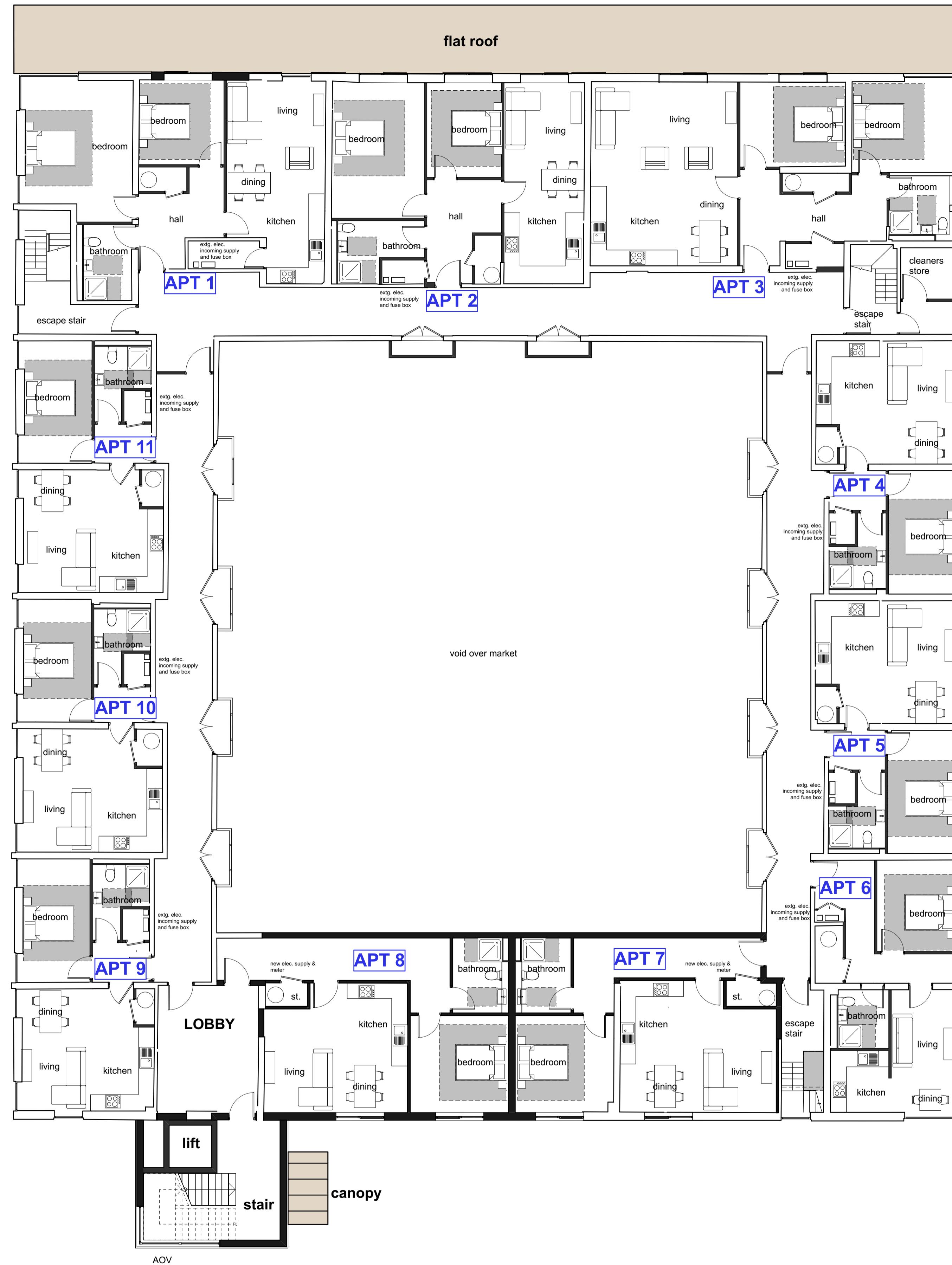
first floor refurb apartments 1:100
