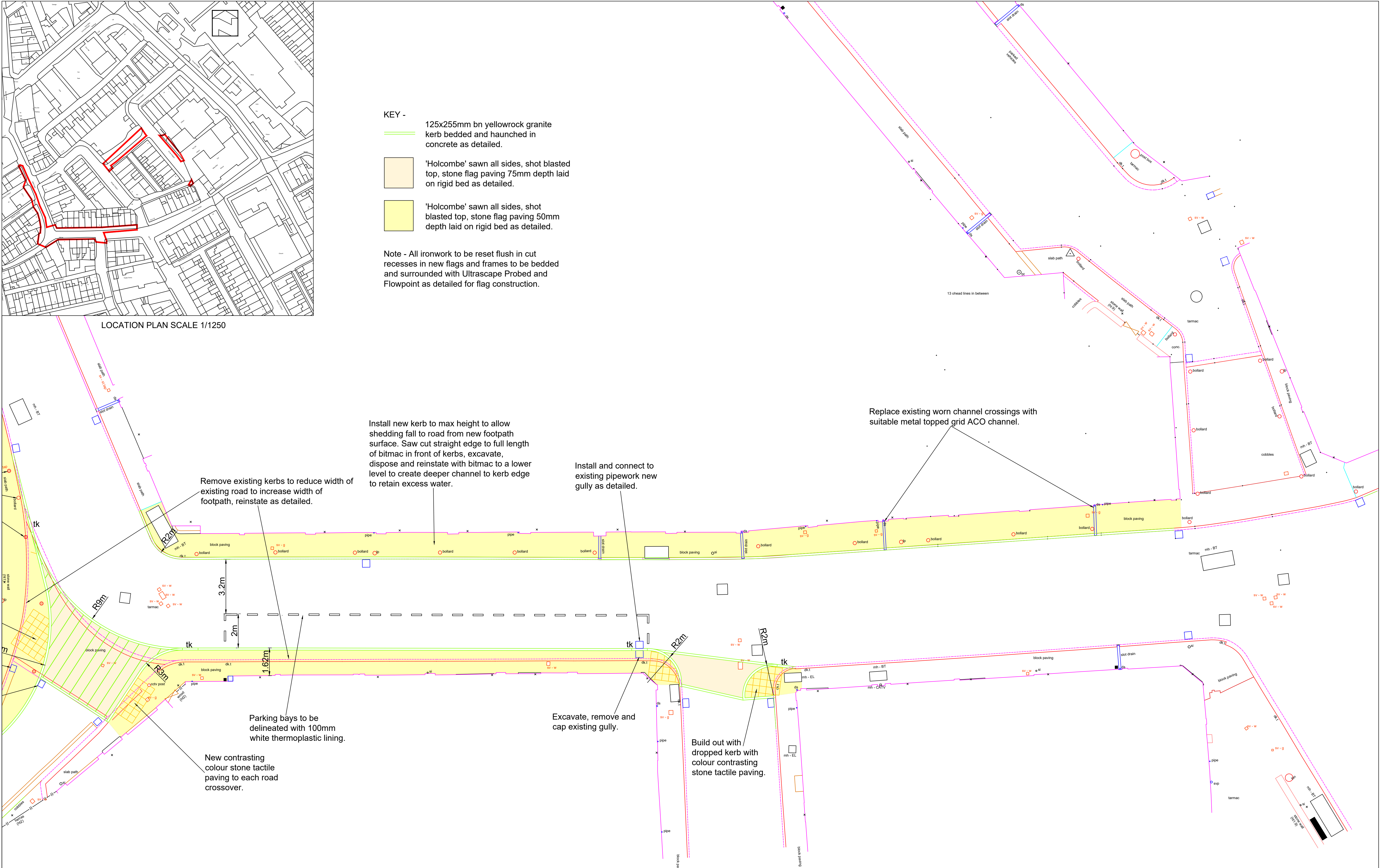
SCHEME DRAWING SCALE 1/100
