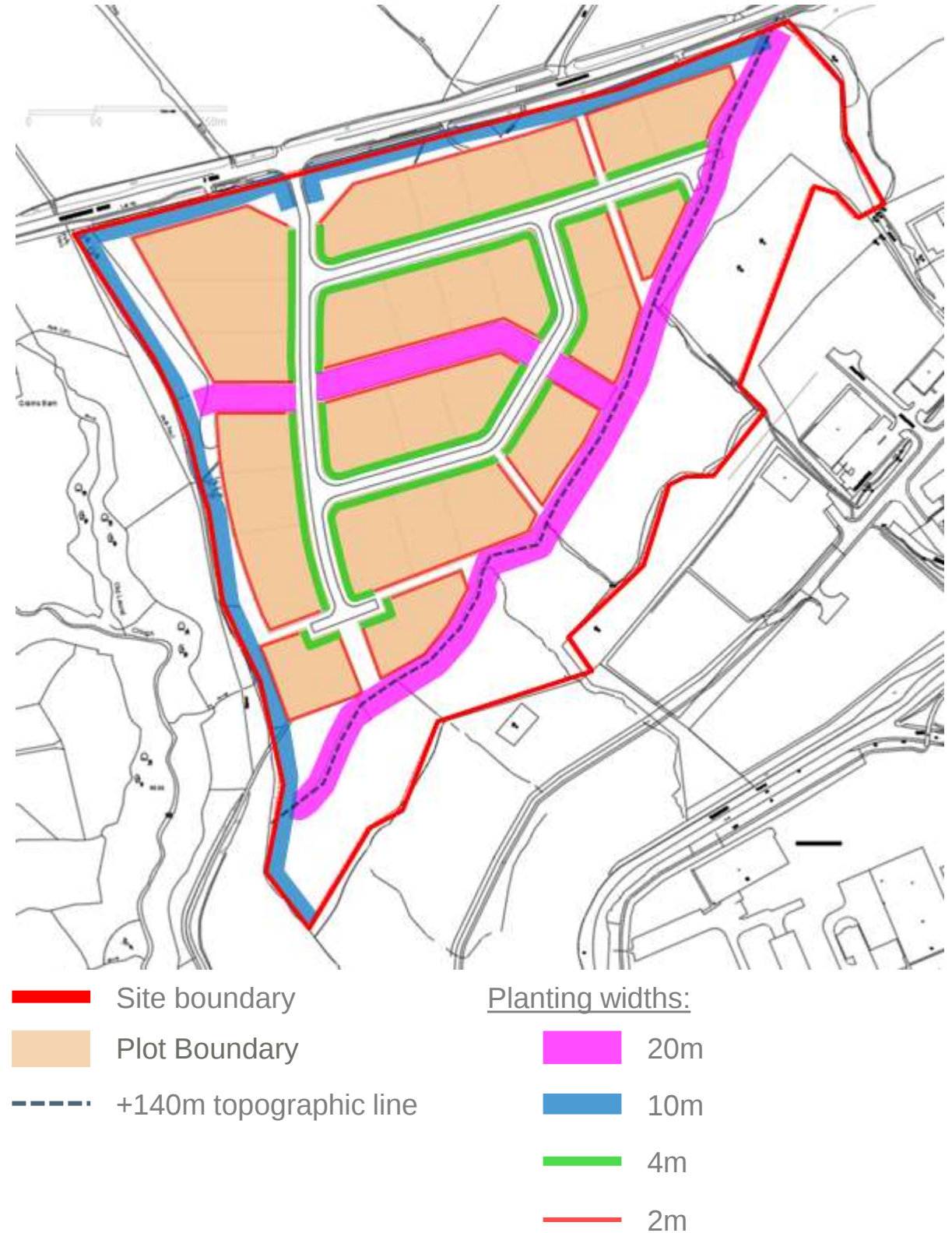
Fig. 10 – Green framework
